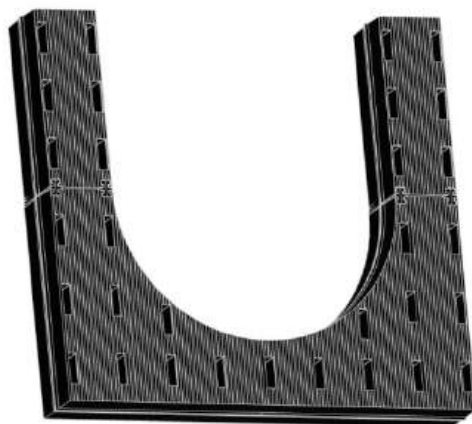
450mm Horseshoe Gully Riser Height = 100mm
